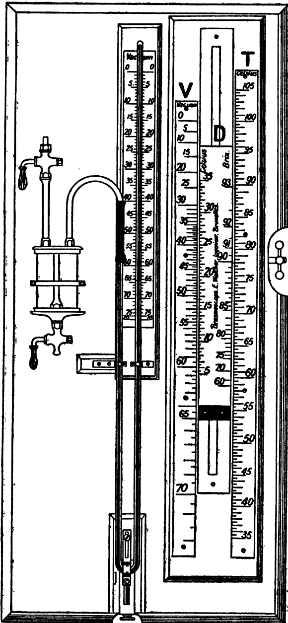
FIG. 34.—BRASMOSCOPE OR BRIXOMETER
